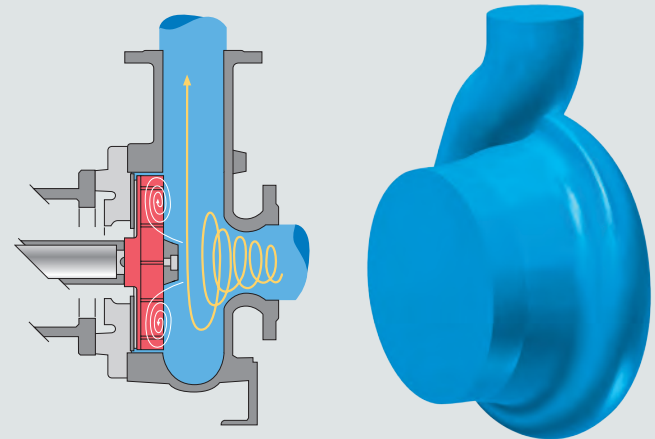
Totally recessed impeller
