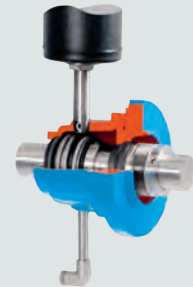
2c. Double mechanical seal in tandem with unpressurised liquid
